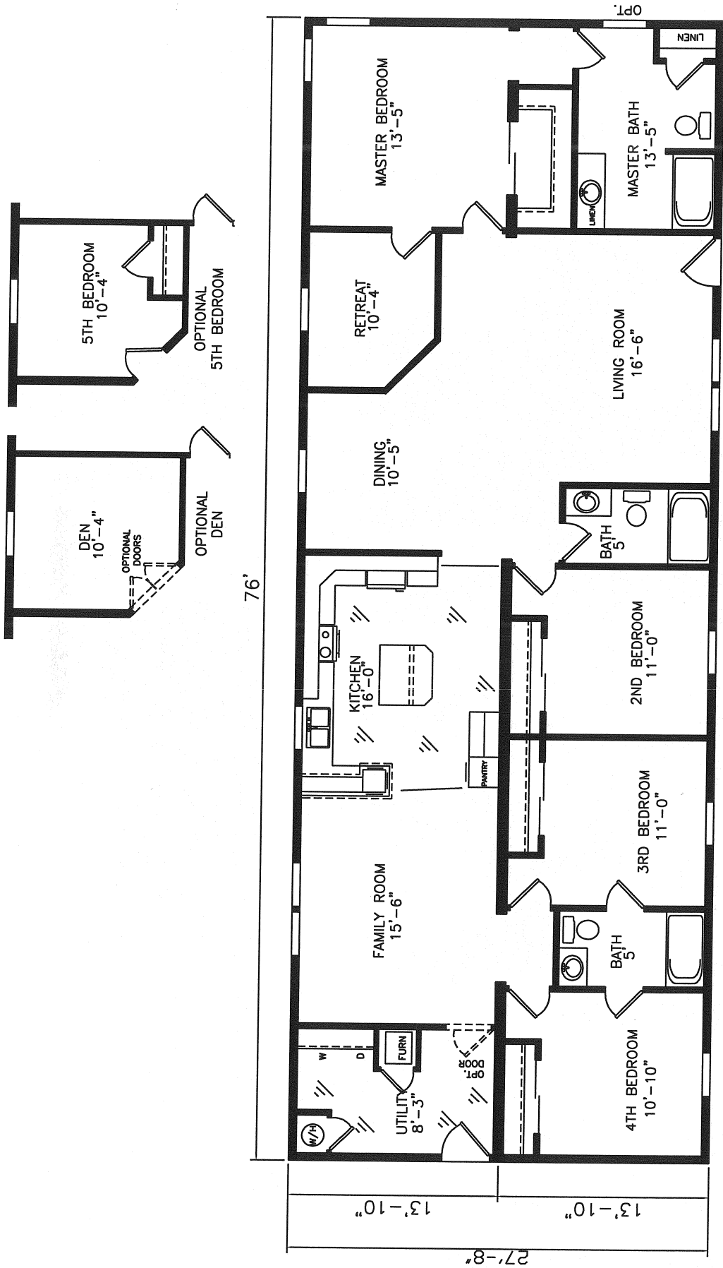
FB-MJ 876 28' X 76' 2105 SQ.FT. FOUR BEDROOM, THREE BATH FAMILY ROOM
